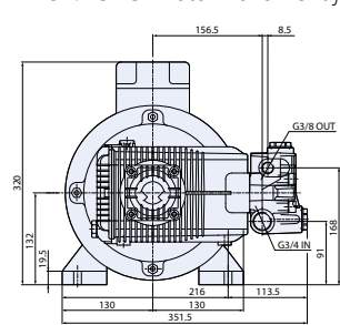
GR. 132 S motor hollow shaft
