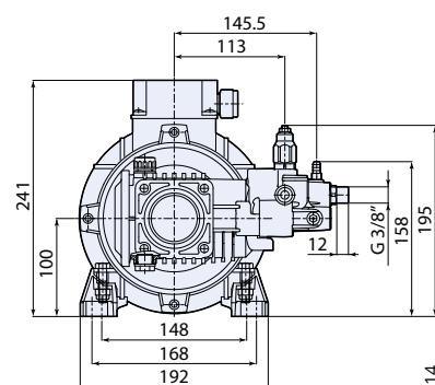
GR. 100 motor hollow shaft
